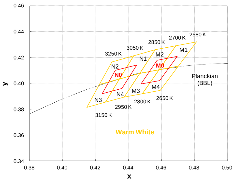
Warm White Binning Structure Graphical Representation
