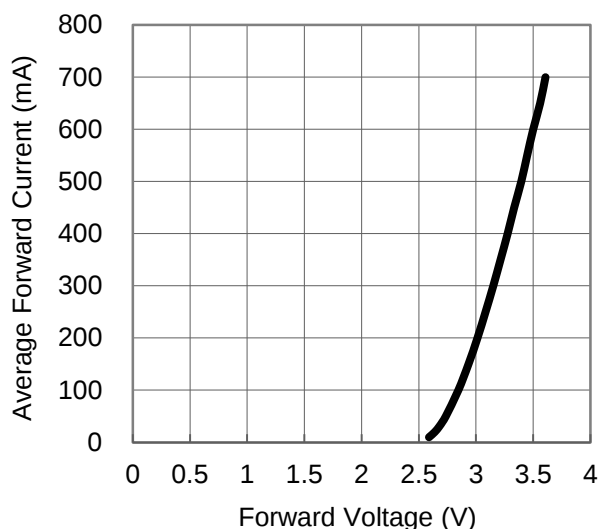
Fig 1. Forward Current vs. Forward Voltage for 2100 K.
