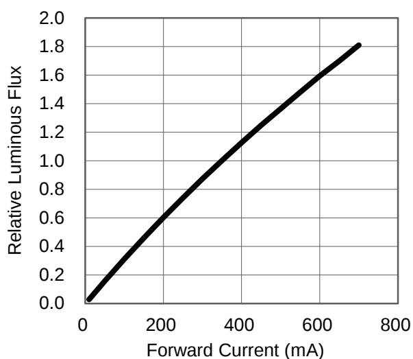
Fig 2. Relative Luminous Flux vs. Forward Current for 2100 K at T_j = 25^\circ\text{C} maintained.
