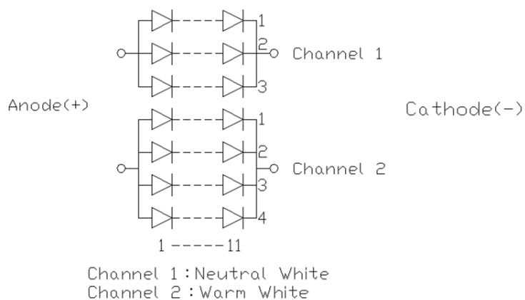
Circuit Diagram
