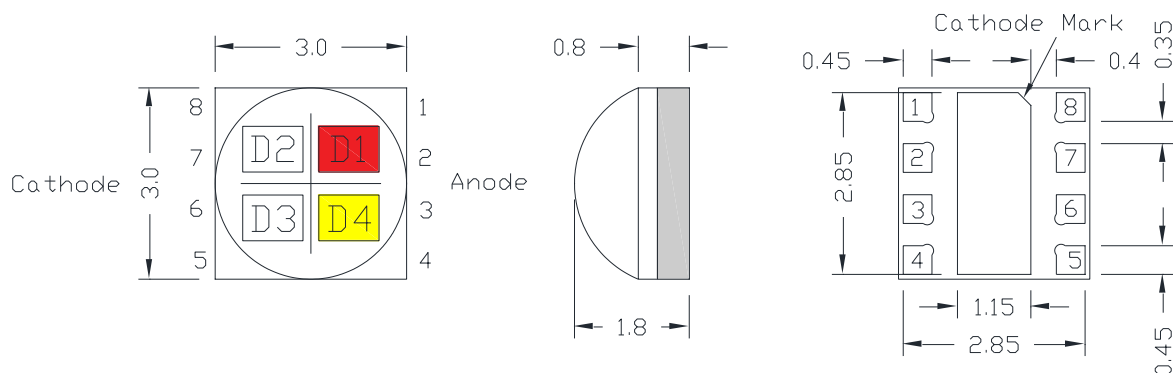
Bottom View
