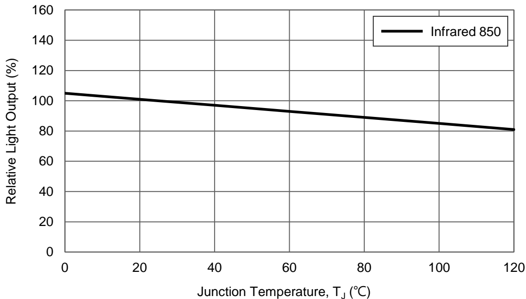
Relative Light Output vs. Junction Temperature at 1500mA
