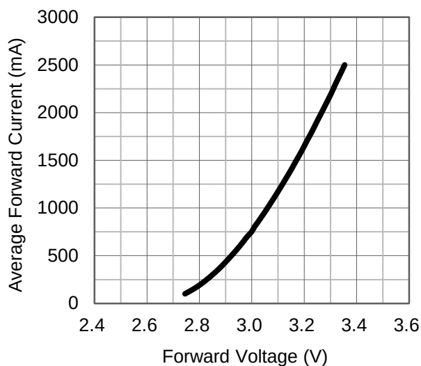
1. Forward Voltage vs. Forward Current
