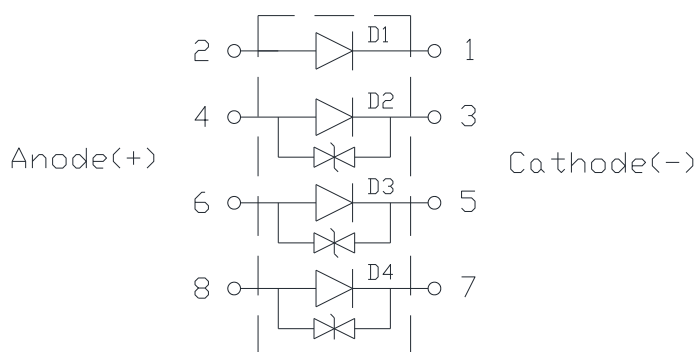
Circuit Diagram
