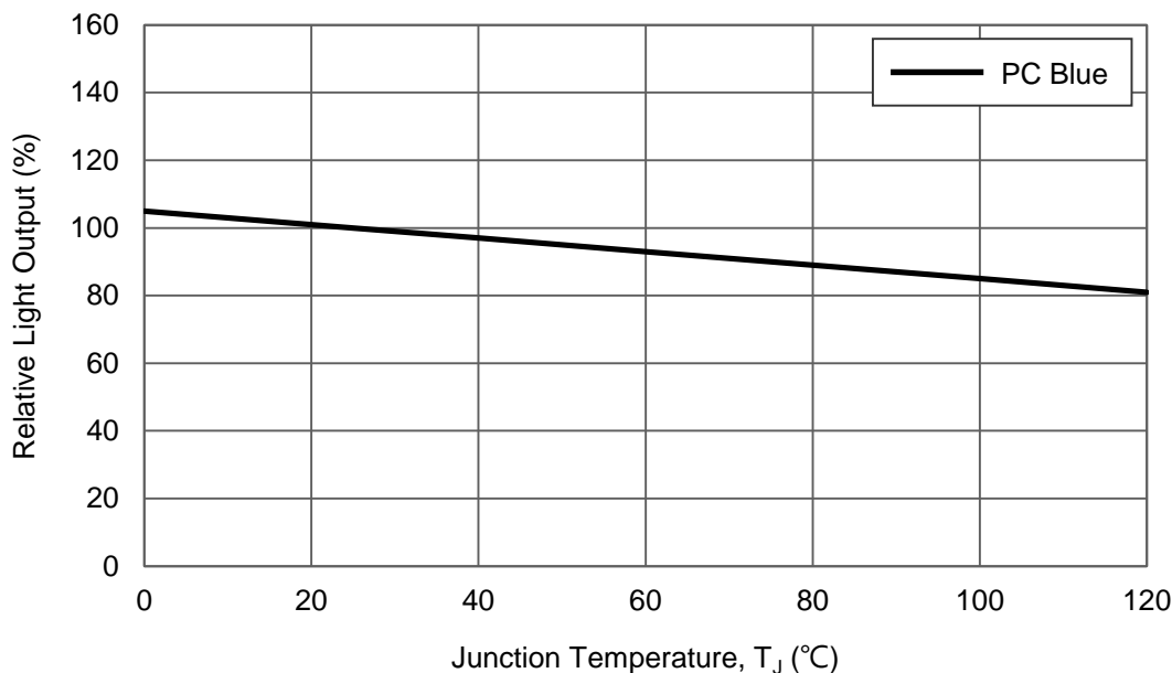
Relative Light Output vs. Junction Temperature at 500mA
