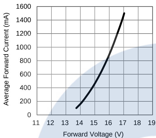
Fig 5. Forward Voltage vs. Forward Current at T_j = 25^\circ\text{C} .
