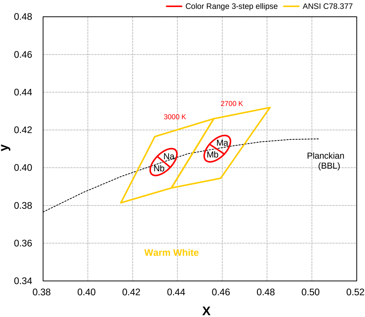
Warm White Binning Structure Graphical Representation
