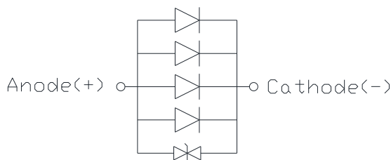
Circuit Diagram
